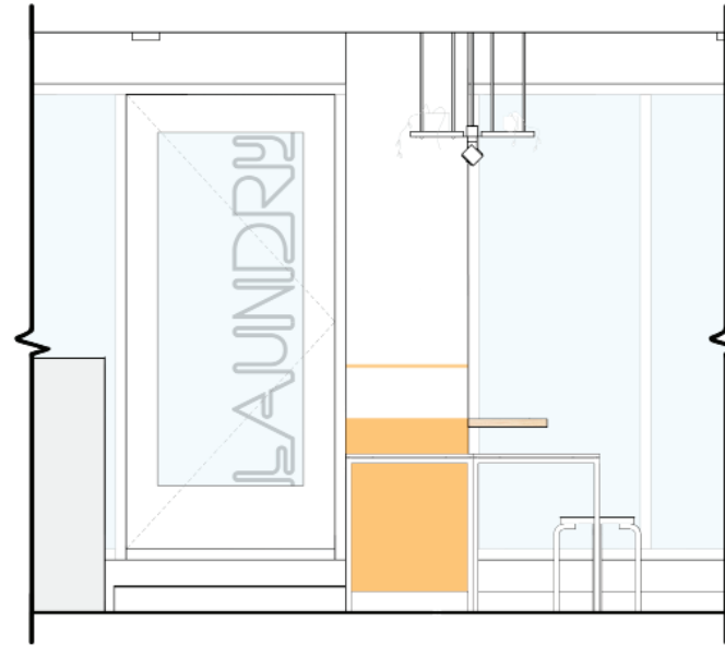
ELEVATION 2 - EXTERIOR CURTAIN WALL
